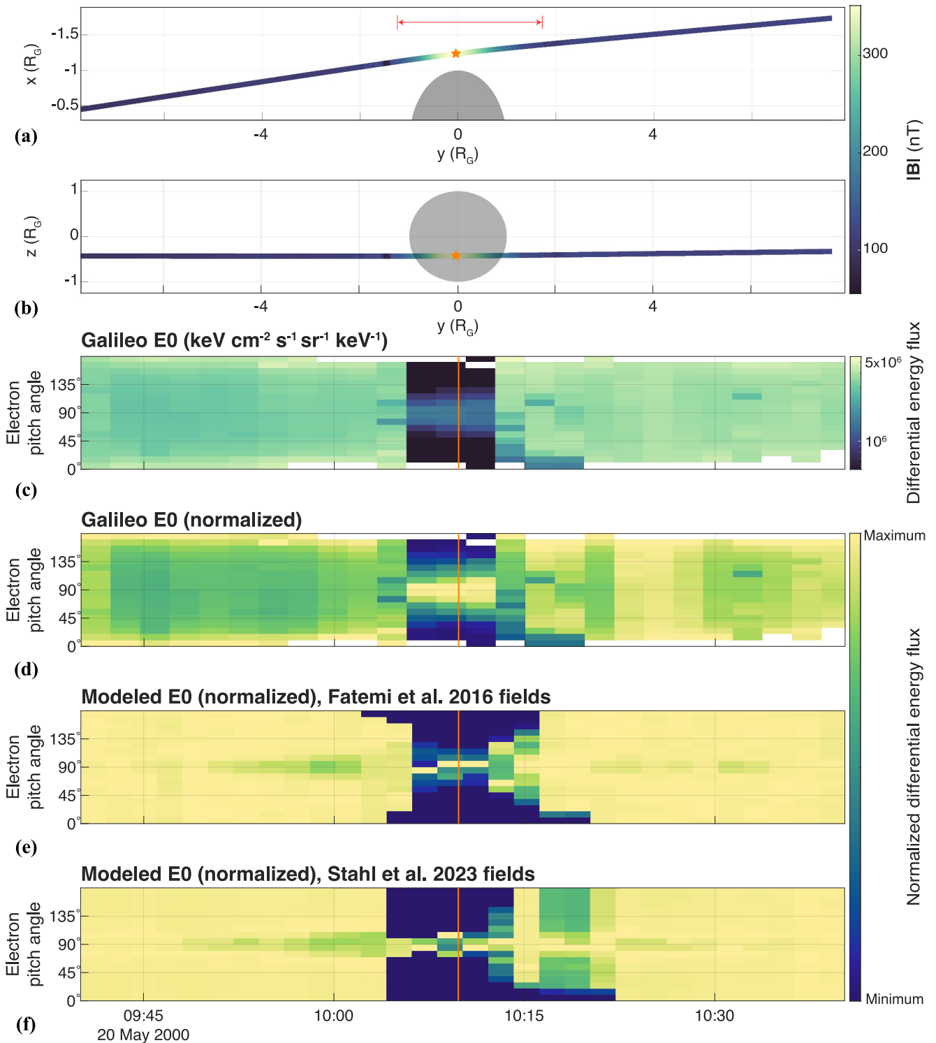
Figure 1. Galileo measurements during G28 and associated model results. Panels (a and b) display the trajectory in the z = 0 and x = 0 planes of the GphiO coordinate system ( x along corotation, z northward), respectively, colored corresponding to the magnitude of the observed magnetic field. Ganymede is represented in gray. Panels (c and d) display the electron pitch angle distribution from the Energetic Particle Detector E0 channel, (c) in units of differential energy flux or (d) normalized to the maximum value of each time bin. Panels (e)–(f) show results from GENTOO, using fields from Fatemi et al. (2016) or Stahl et al. (2023b), respectively. The temporal position of each bin in panels (c–f) corresponds to the spatial position of Galileo in panels (a) and (b). Orange stars and vertical lines denote C/A, while the red horizontal line in panel (a) indicates the closed magnetic field line region (Kivelson et al., 2002; Williams, 2001).
