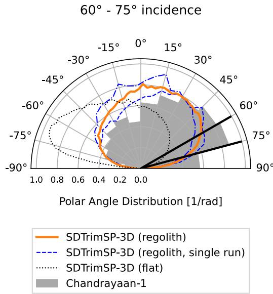
Figure 1. Polar angle distributions from SDTrimSP-3D show clear differences between the scattering behavior from a flat surface (dotted black line) and from the porous regolith (orange, compiled from five different regolith simulations). For the ion incidence between 60° and 75° (marked by the full black lines), significant forward scattering (negative angles) would be expected from a flat surface. However, the regolith surface shows a backward-dominated scattering behavior, which agrees with the Chandrayaan-1 observations of the Energetic Neutral Atom scattering function from the lunar surface (gray, from Schaufelberger et al. (2011)). The blue lines furthermore give two examples of single simulation runs at 70° incidence to illustrate that the scattering angles can vary for different regolith structures.
