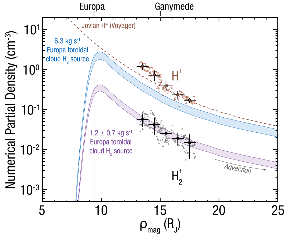
Figure 2. Partial density of \text{H}_2^+ pickup ions (gray) and \text{H}^+ (orange), with average values every 1 R_J for \epsilon = 1.2 . The blue curves show expected \text{H}_2^+ pickup ion densities for a neutral Europa loss \text{H}_2 rate of 6.3 \text{ kg s}^{-1} (Smyth & Marconi, 2006). The purple curves show the best fit solution to the observed \text{H}_2^+ partial densities. These observations are consistent with a Europa neutral \text{H}_2 loss rate of 1.2 \pm 0.7 \text{ kg s}^{-1} . The orange dashed line shows an empirical model for proton densities based on Voyager observations (Bodisch et al., 2017).
