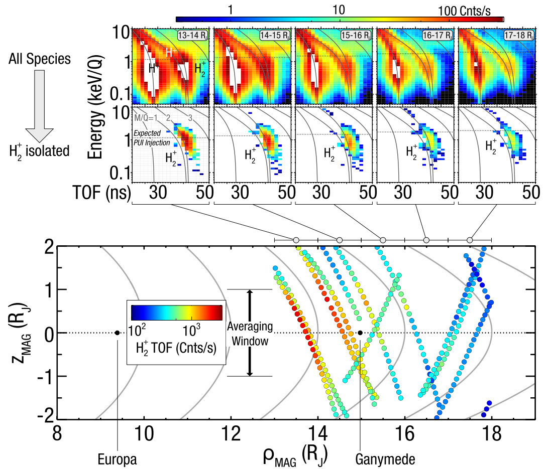
Figure 1. Count rates of \text{H}_2^+ from 13 to 18 R_J (top) Ion energy per charge as a function of time-of-flight (TOF) for all species with nominal background subtraction (upper row) and with \text{H}_2^+ isolated (lower row) for all observations within an averaging window of \pm 1 R_J from the magnetic equator. \text{H}_2^+ is unambiguously observed when foregrounds and backgrounds are removed, in the vicinity of the second gray TOF trace for a mass per charge of 2. The horizontal line indicates the expected detected energy for a freshly created pickup ion at the spacecraft's position (bottom) Locations of each observation in cylindrical coordinates with the +z axis are aligned with Jupiter's magnetic dipole. \text{H}_2^+ is observed with the strongest magnitude in the inner-most detected locations.
