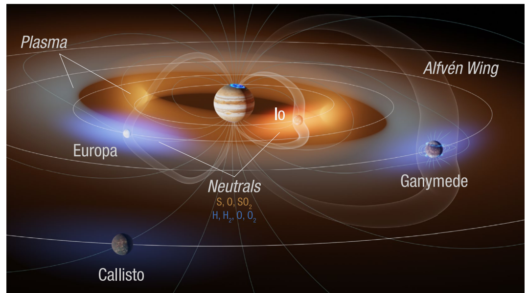
Figure 3. Overview of Jupiter's magnetosphere in the vicinity of the Galilean satellites. H 2 + pickup ions (blue) originate from Europa's neutral toroidal cloud (brighter blue near Europa). Io and Europa contribute plasma pickup ions of different compositions to Jupiter's magnetosphere. Alfvén wings connected to the moons due to their interaction with corotating plasma are also shown in gray.
