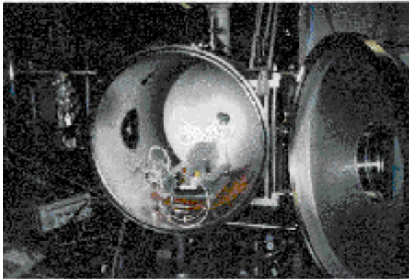
Above: A vacuum chamber at the Space Sciences Laboratory used to test the Mars Microphone.
