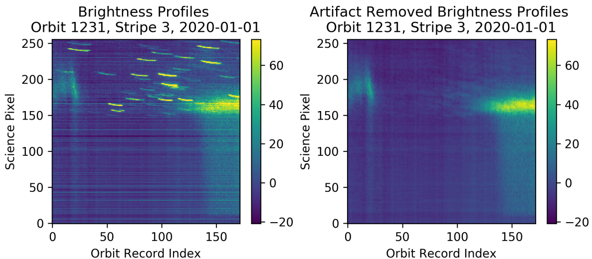
Fig 5.9: Demonstration of stellar track removal applied in the course of FUV Level 1 processing.
