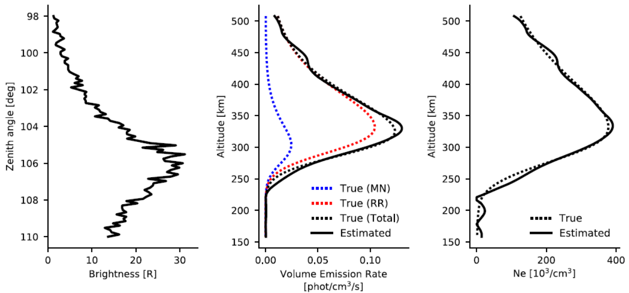
Fig 5.5: Example of an end-to-end ICON FUV inversion corresponding to 10 PM local time at 0 degrees latitude, 0 degrees longitude. Left panel: simulated FUV brightness as a function of zenith angle based on an IRI electron density profile and corresponding volume emission rate using MSIS and 135.6 nm emission containing radiative recombination and mutual neutralization. The simulated brightness was obtained based on ICON FUV viewing geometry and instrument characteristics. Middle panel: solid black curve shows the reconstructed volume emission rate from the simulated brightness of the left panel. Dotted black curve shows the original (simulated) true volume emission rate. The dotted red and blue curves show the contributions from radiative recombination and mutual neutralization processes respectively which in combination result in the total simulated volume emission rate in dotted black curve. Right panel: Solid curve shows the reconstructed electron density profile in comparison with the dotted line which shows the simulated (true) profile
