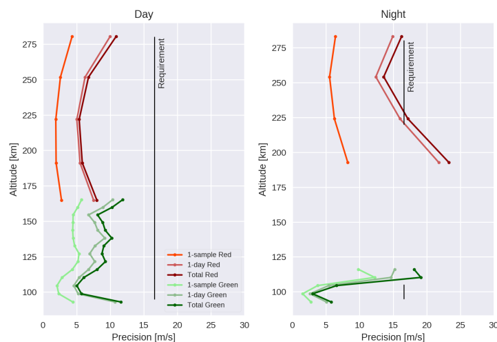
Fig 18: MIGHTI-A and MIGHTI-B averaged precision numbers for 24 days in early 2021. The vertical line indicates the ICON wind precision requirements and corresponding altitude regions. Values are determined for a horizontal resolution of <500 km and the vertical resolutions of 30 km (5 km) for the middle (lower) thermosphere, corresponding to the ICON mission requirements.
