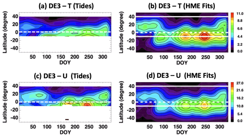
Fig 16: MIGHTI DE3 amplitudes in (a) temperature and (c) zonal wind at 98 km in 2021. Amplitudes of DE3 HME fits in (b) temperature and (d) zonal winds at 98 km in 2021.
