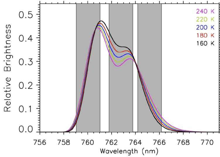
Fig 14: Curves illustrate the temperature dependence of the oxygen A-band. The gray areas indicate the MIGHTI on-band filter positions (doi: 10.1007/s11214-017-0434-9).
