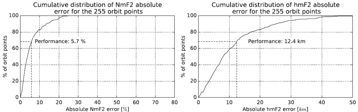
Fig 5.8: Cumulative distribution function of errors in NmF2 and hmF2 calculated for each of the 255 points in the orbit, whereby the fraction (%) of orbit points within an error range is depicted. Note that 1 standard deviation (1-sigma) value corresponding to a normal distribution is shown with the dashed lines for both NmF2 and hmF2, and both fall well within the requirements
