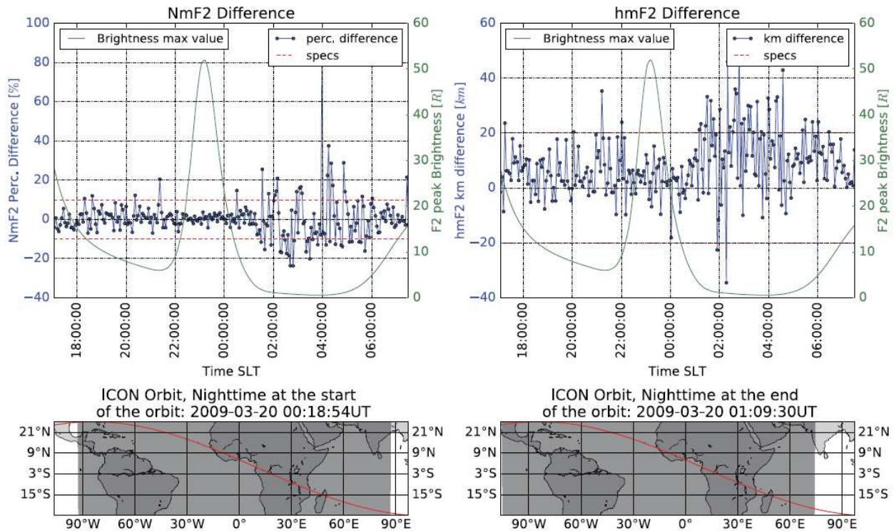
Fig 5.6: An ICON partial orbit containing 255 orbit measurement points, spanning from -100 to 100 degrees longitude and -20 to 22 degrees latitude is shown in the bottom panels. The green line shows the simulated peak brightness ( R ) using ICON FUV instrument characteristics (sensitivity). The volume emission rate is reconstructed from the simulated brightness for each point in the orbit and the electron density is calculated followed by extraction of the F2 peak parameters and comparison with the “true” (original) F2 peak parameters of the electron density simulated from the IRI model. The top panels show the resulting errors in NmF2 and hmF2 for each measurement (in blue) and the ICON requirements (in red). As can be seen from the figure, the reconstruction errors are within the requirements (20 km for hmF2, 10% for NmF2, Immel et al. (2018) for time intervals when there is sufficient signal
