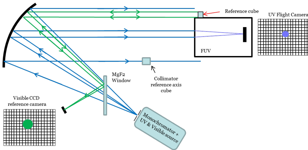
Fig 4.1: Overall setup for the alignment of the ICON-FUV instrument.
