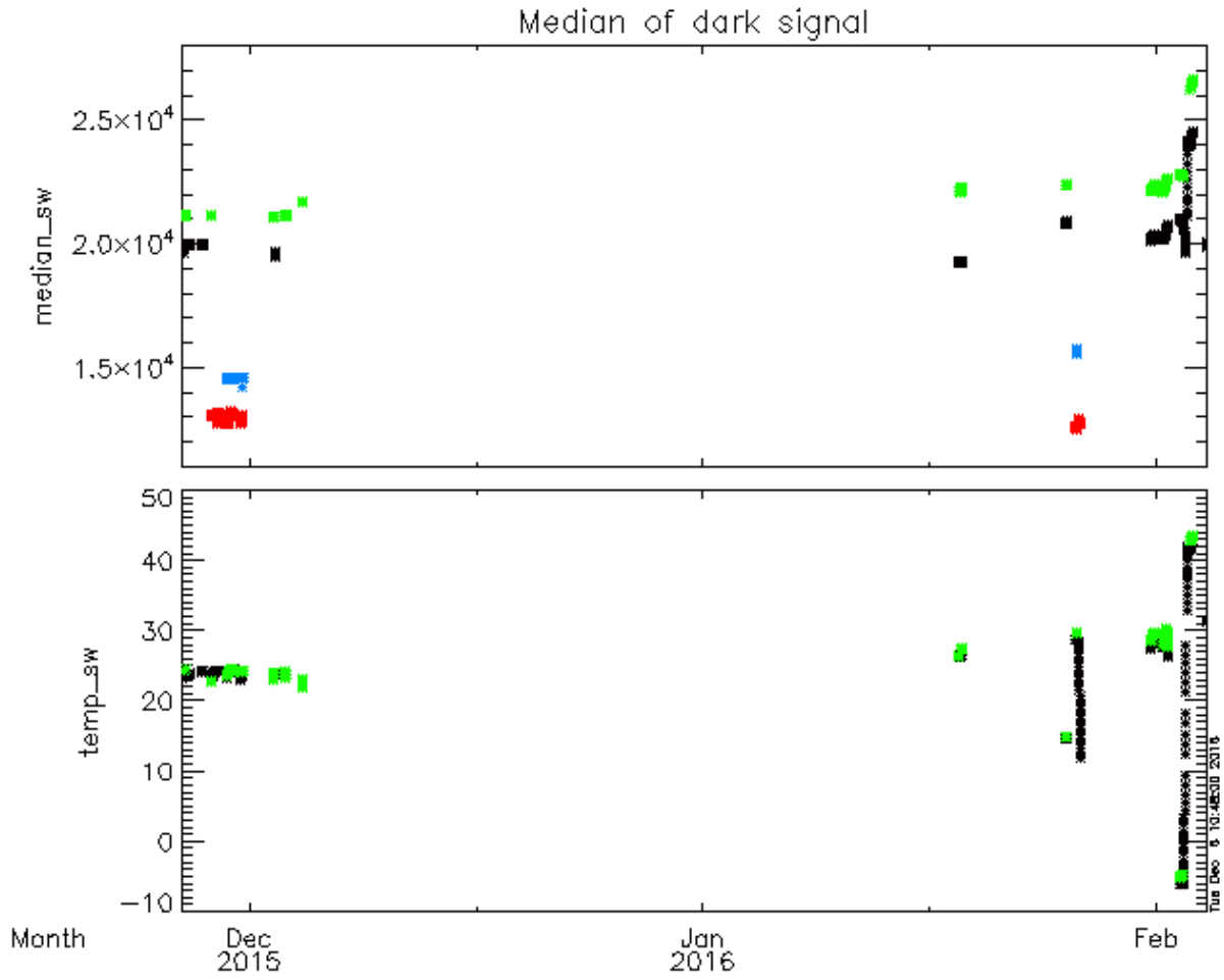
Fig 4.45: Summary of all measurements used for the dark signal determination. The horizontal axis is the date of the tests. The top plot shows the median values of the dark signal across the whole image (536x515 engineering images) for the two channels. Details about the colors are given in the text. The bottom plot shows the CCD temperatures at the time of the measurements, the black symbols for SW and the green symbols for LW.
