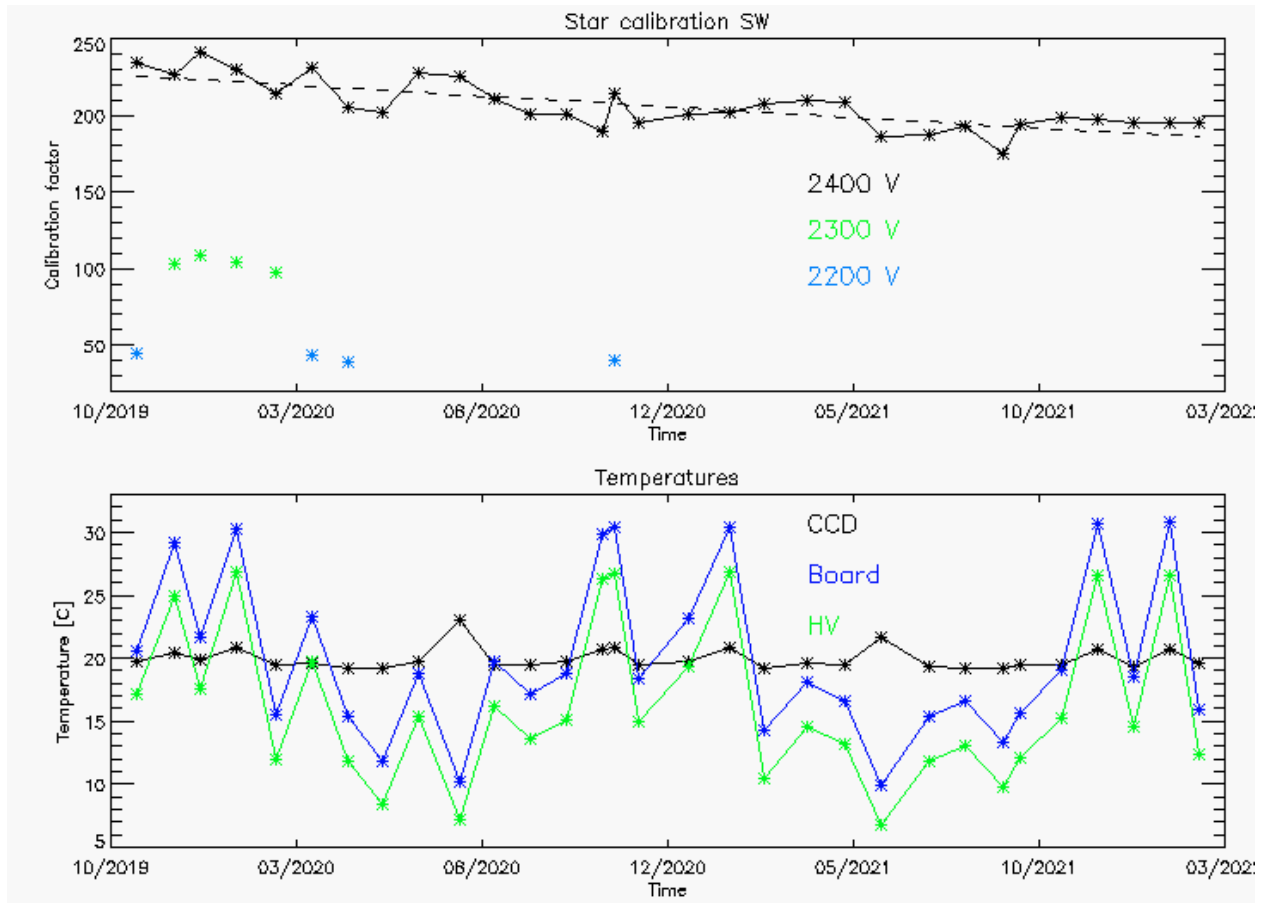
Fig 5.3: Results of the star calibrations during the first 2.5 years of the ICON mission for the SW channel. The calibration factors of Counts/s are shown over time as well as temperatures of key components of the detector system that could have an impact on the relative response.
