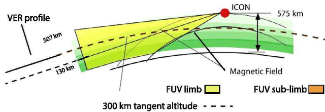
Fig 3.1: Side view of ICON FUV viewing geometry (not to scale). ICON S/C is shown travelling into the page (eastward) on the magnetic equator at 575 km altitude with FUV viewing on the port side with the central ray observing at 20 degrees below local horizontal. Volume Emission Rate (VER) profile with altitude for nighttime 135.6 nm emission shown on left
