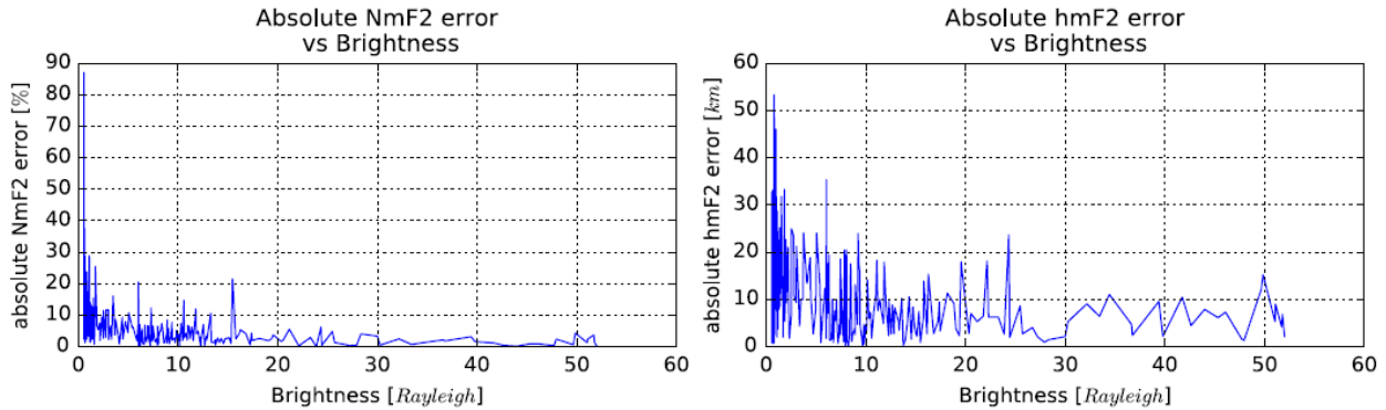
Fig 5.7: NmF2 and hmF2 errors for the 255 orbit points as a function of the simulated brightness. This figure exhibits the correlation between source brightness and reconstruction error. For brightness values above 10 R, the reconstruction errors are within the specified specifications of the ICON mission for both NmF2 and hmF2
