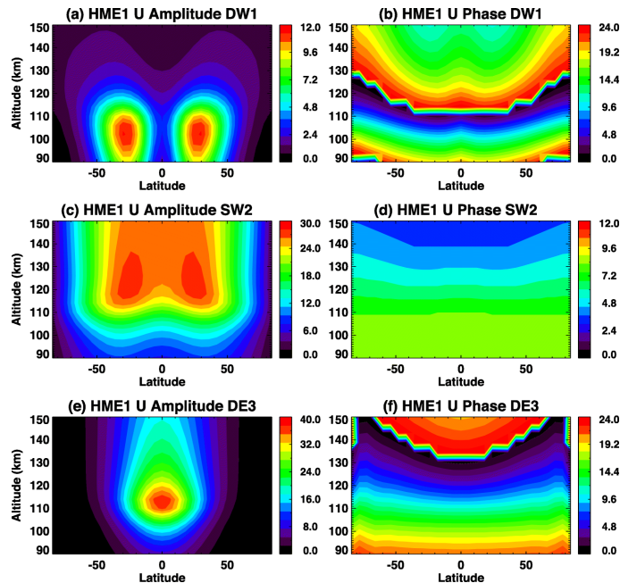
Fig 15: First symmetric HME amplitudes and phases for zonal wind ( U ) for a, b DW1; c, d SW2; and e, f DE3. HMEs are arbitrarily calibrated in amplitude to yield a maximum perturbation horizontal wind speed of 10 m/s (either zonal or meridional, whichever is larger) at 93 km. Absolute values of phases are also arbitrary.
