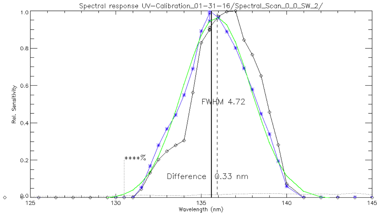
Fig 4.21: Spectral scan measurements on 2016-01-31 at room temperature. The black line with diamonds shows the raw measurements normalized to the maximum counts. The black dotted line is the source meter reading normalized to its maximum around 161 nm. The blue line with asterisks is the counts divided by the source meter current reading normalized to the maximum of that ratio. The green line is a Gaussian fit to the normalized measurements. The maximum of the fitted Gaussian is at 0.33 nm higher than the target wavelength of 135.6 nm. The FWHM of the Gaussian is 4.72 nm. The 130.4 response is basically zero.
