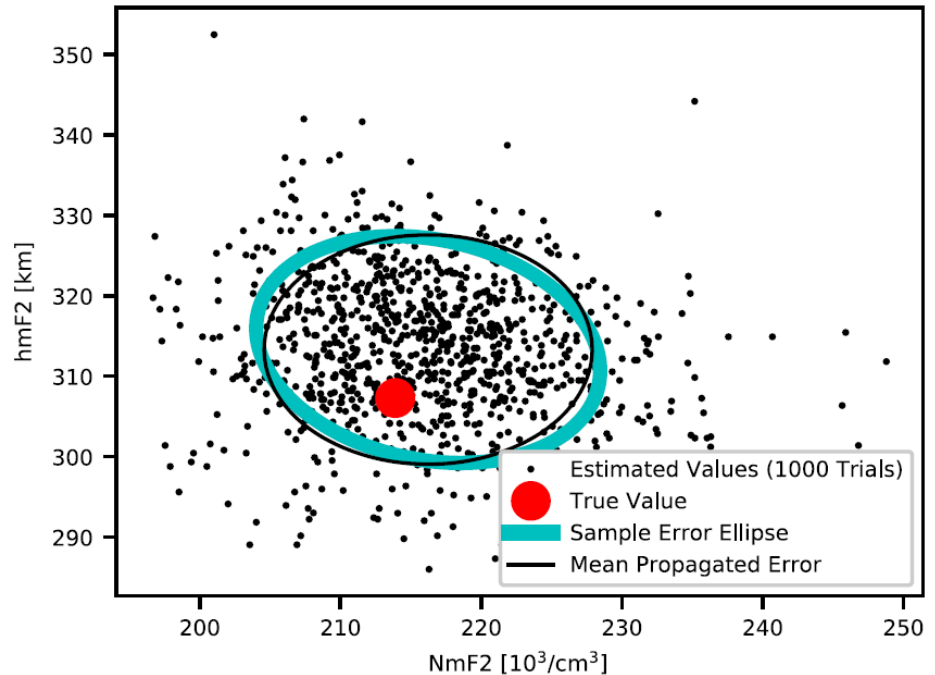
Fig 5.4 The error propagation algorithm is validated with a Monte Carlo simulation. A model electron density profile is used to simulate 1000 noisy measurements, from which 1000 samples of hmF2 and NmF2 are generated. The covariance ellipse of these samples is compared to the mean propagated error
