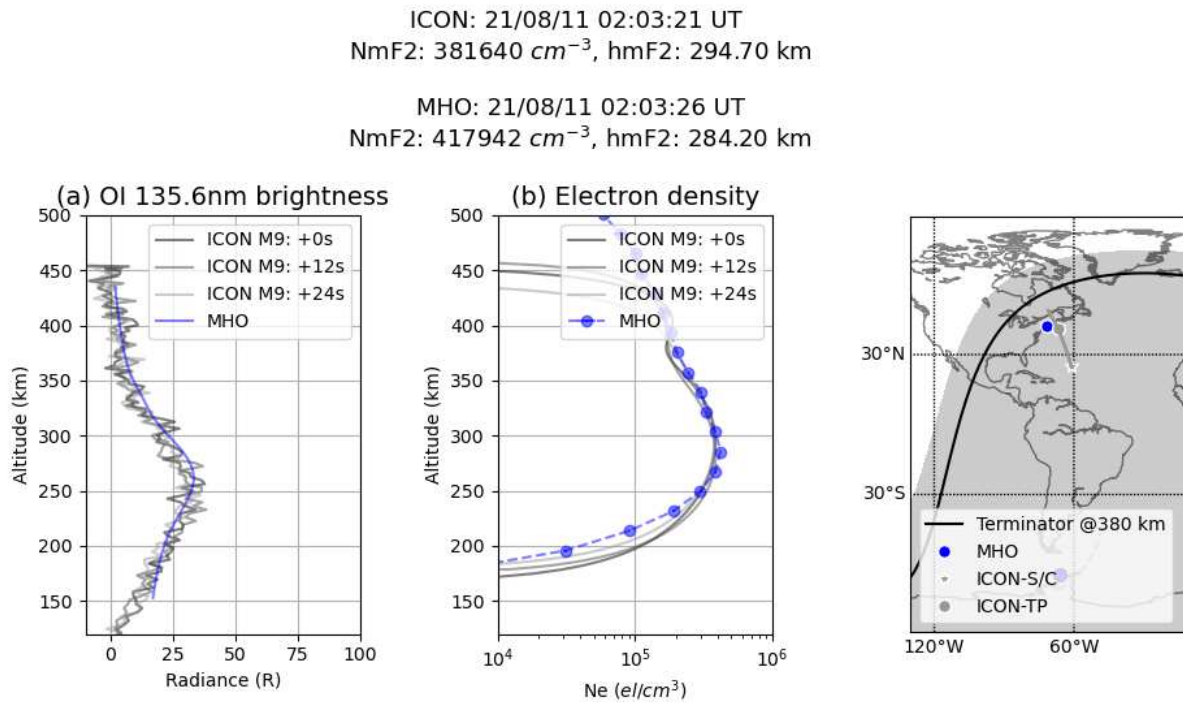
Fig 4.69: Comparison between nightside measurements of ICON-FUV and the Millstone Hill Incoherent Scatter Radar (MHO). The derived ionospheric peak densities agree within 10% and the peak altitude difference is within the radar altitude resolution.
