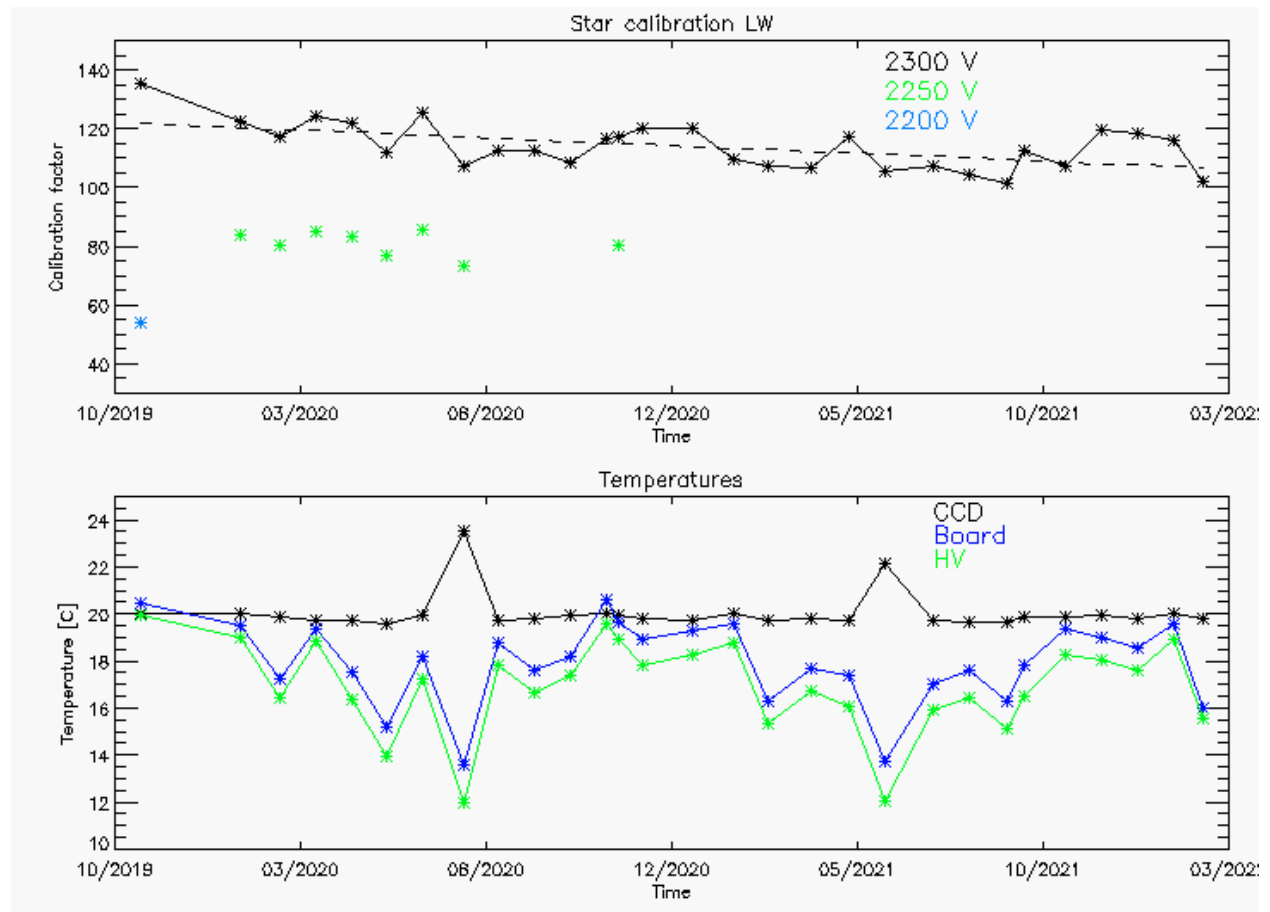
Fig 5.2: Results of the star calibrations during the first 2.5 years of the ICON mission for the LW channel. The calibration factors of Counts/s are shown over time as well as temperatures of key components of the detector system that could have an impact on the relative response.
