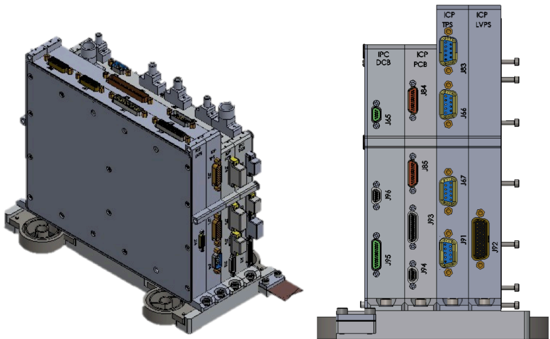
Fig. 13 The ICON ICP, with four main boards in aluminum housings on a flexure mount, provide all necessary functionality for the 4 ICON science instruments, and a single point interface to the
