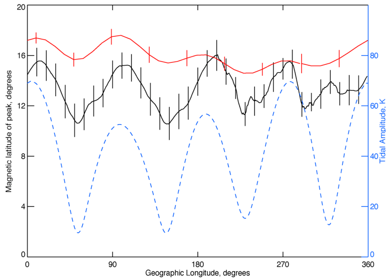
Fig. 3 Longitudinal variations in the nighttime FUV brightness of the equatorial ionospheric anomaly compared to the amplitude of predicted temperature variations driven by non-migrating diurnal tides at the equator. The FUV emissions originate from the F-layer of the ionosphere above 300 km (from IMAGE FUV (black) and TIMED GUVI (red)), while the temperature amplitudes from the Global Scale Wave Model are shown at 115 km (blue). After Immel et al. , 2006.
