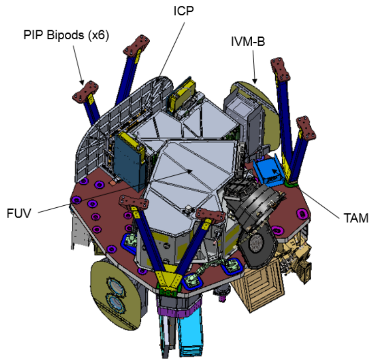
Fig. 14 a, b A model of the ICON science payload, viewed from a point above its Earth-facing side (Fig. 14a), and also from the side that will face the spacecraft (Fig. 14b). Each instrument and components are noted. The two star trackers (CHUs) are found on either side of the EUV instrument, also visible in Figure 15.
