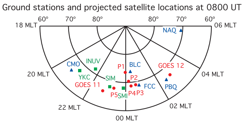
Figure 5. A map of ground stations and projected satellite locations at 0800 UT. The ground stations contributing to the AU/AL indices are marked by solid triangles. The THEMIS GBO stations used in this study are marked by solid squares. The projected satellite locations based on the T89 magnetic field model are marked by solid circles.
