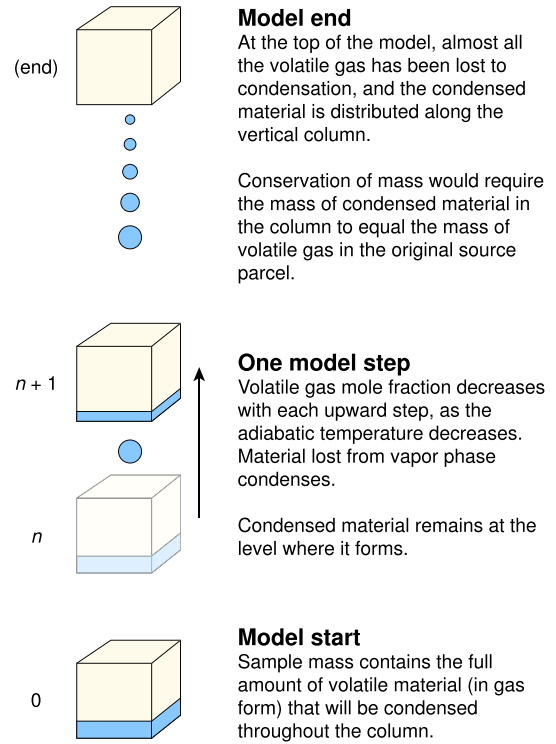
Fig. 1. Overview of the equilibrium cloud condensation model's treatment of volatile material.
