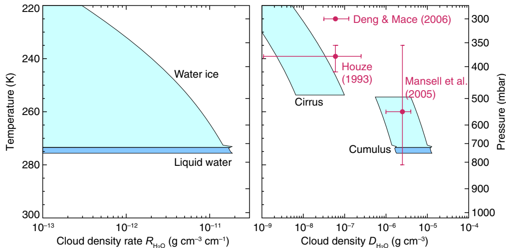
Fig. 4. Fresh cloud model density rates R_{H_2O} (left) and cloud densities D_{H_2O} (right) for Earth, compared with terrestrial cirrus and cumulus observations. Model initial conditions include standard atmospheric temperature and pressure (298.15 K, 1 bar), and a composition of X_{H_2O} = 1\% (99% dry air). The arc-shaped spread in densities at each level covers a range of updraft length scales for cirrus corresponding to updraft speeds of 0.02\text{--}0.2\ m\ s^{-1} over a duration of 10–15 min. For cumulus, updraft speeds are 1\text{--}5\ m\ s^{-1} for a duration of 16–23 min (Houze, 1993). Model calculations agree very well with observations of typical cirrus (Houze, 1993) and with cumulus formed in a 3D fluid model (Mansell et al., 2005). Model densities under-predict observations of a tropical anvil cirrus (Deng and Mace, 2006), partly due to neglect of transport and partly due to slower updraft velocities in the model. Vertical temperature and pressure axes are the same in both panels.
