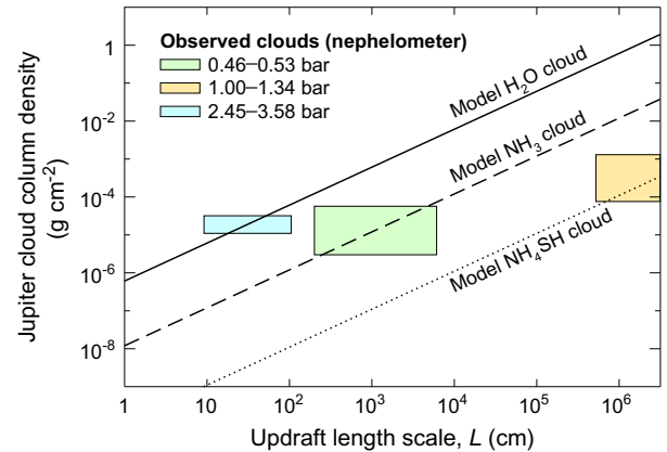
Fig. 5. Comparison between observed clouds in the Galileo Probe entry site and modeled fresh clouds. Observed cloud column densities (vertical extents of the shaded boxes) are based on nephelometer measurements integrated over the given pressure ranges (Ragent et al., 1998). Model cloud column densities for each cloud composition are given by the slanted lines, as a function of updraft length scale L . Model cloud column densities are calculated for the same pressure ranges as the observed clouds; column density rate is the value of each line as it crosses L = 1 cm. Updraft length scales thus correspond to the intersections of the lines and boxes.
