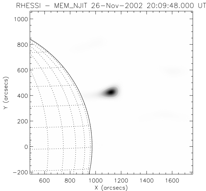
Figure 6. Five-hour long RHESSI image, from 2002/11/26 20:10 to 2002/11/27 01:10 UT, in the 4–8 keV energy band. RHESSI visibilities were generated in 5 minute accumulations, then bundled together after shifting their phases to remove source motion effects (relative to the source position at 20:09:48 UT).
