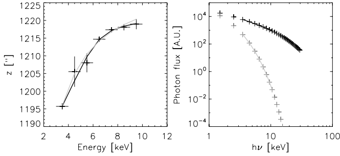
Figure 8. Left: crosses: positions of emission at different energies, with error bars (vertical lines) and bin widths (horizontal lines). Solid black line: fitting to the Gaussian T and exponential EM profiles. Solid gray line: same, with T fixed to 10 MK. Right: crosses: synthetic X-ray spectra generated using the fitting parameters found. Solid line: fit to the crosses in the 4–10 keV band. Color scheme same as in the plot on the left. See the text for more details.
