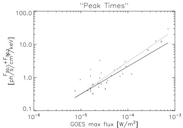
Figure 9 GOES maximum flux in the 1–8 Å band versus peak 50-keV flux of both footpoints, with 1- \sigma errors. The solid line is a power-law linear fit to the data. The dotted line is another power-law fit to the data, using the bisector method.
