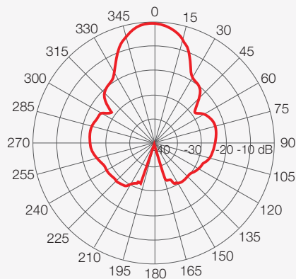
Figure 1. Displayed on a horizontal plane, this measurement shows the far-field antenna pattern of an X-band radar. Source: Figure 50, pg 65, 5989-7575EN
